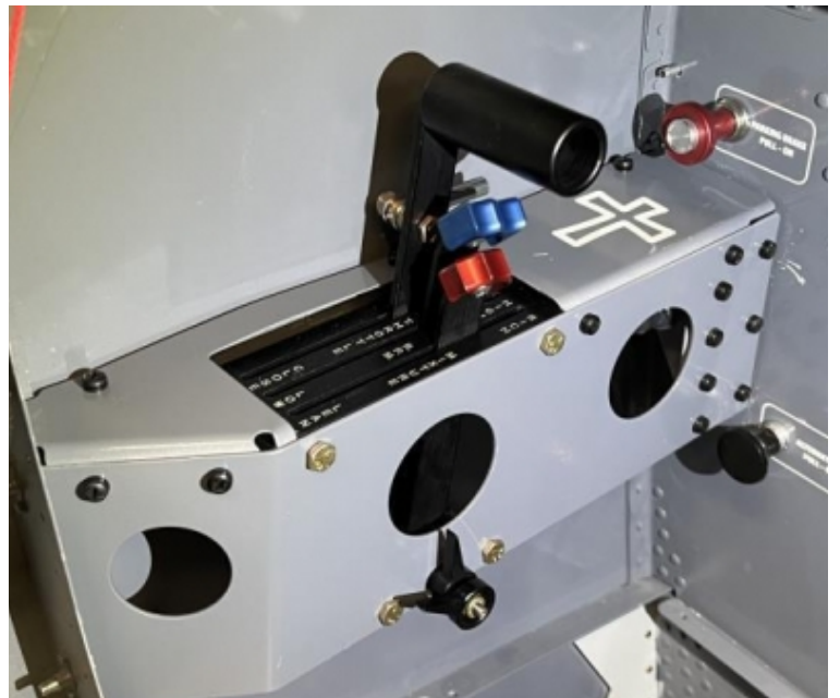
Jim Novak's RV-8 Throttle Quadrant installed
