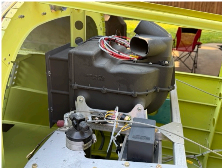
RV-10's Evaporator assembly
