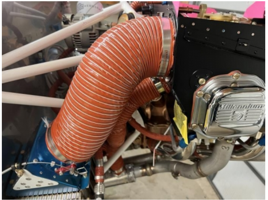
Remote mounting the Oil Cooler on an RV-8
